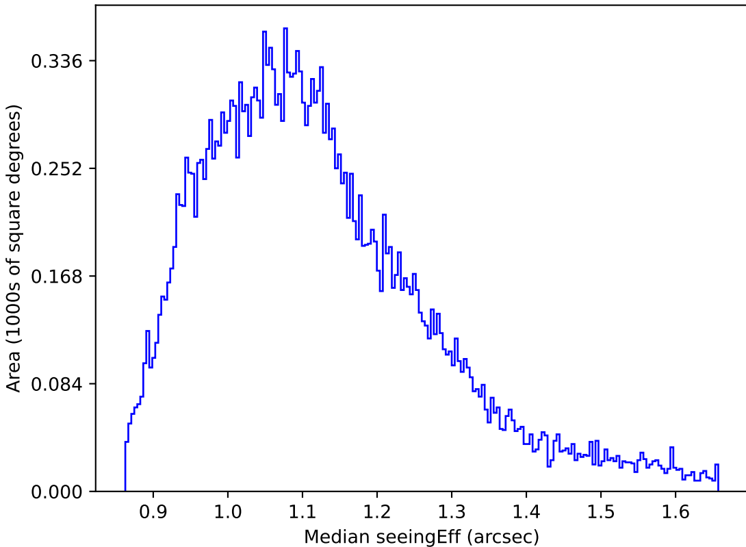
no_high_blob_v3.3_10yrs All sky g band: Median seeingEff
