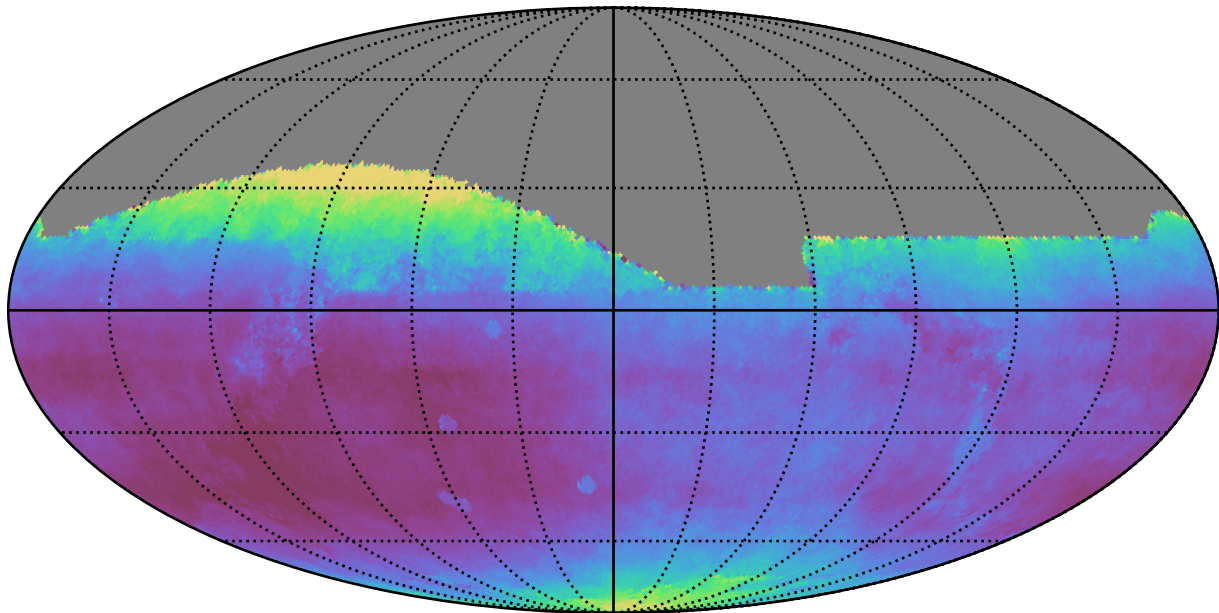
no_high_blob_v3.3_10yrs All sky all bands: Median seeingEff
