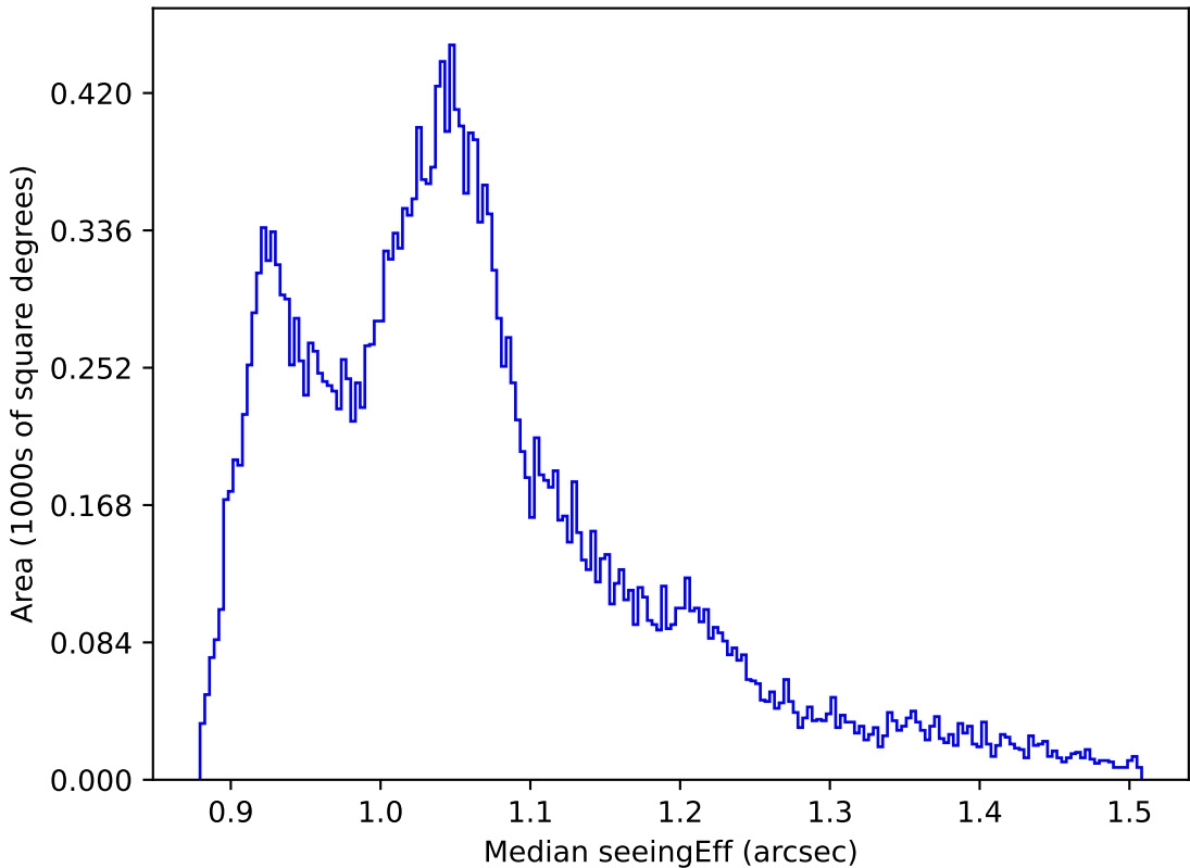
no_high_blob_v3.3_10yrs All sky all bands: Median seeingEff
