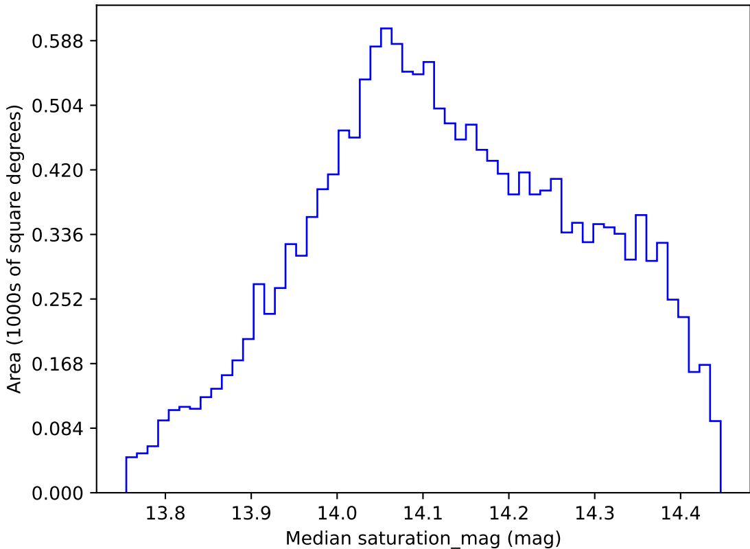
no_high_blob_v3.3_10yrs WFD z band: Median saturation_mag
