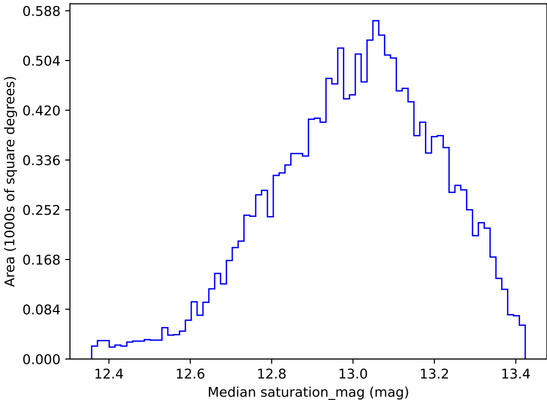
no_high_blob_v3.3_10yrs WFD u band: Median saturation_mag
