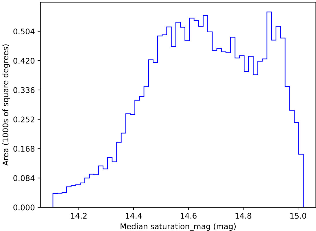
no_high_blob_v3.3_10yrs WFD r band: Median saturation_mag
