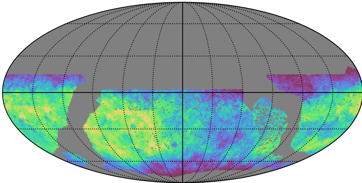
no_high_blob_v3.3_10yrs WFD g band: Median saturation_mag
