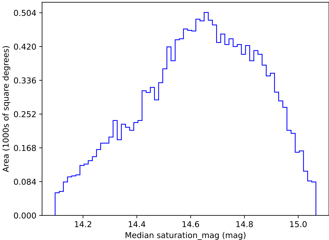
no_high_blob_v3.3_10yrs WFD g band: Median saturation_mag
