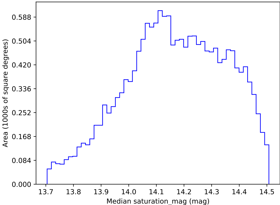
no_high_blob_v3.3_10yrs WFD all bands: Median saturation_mag
