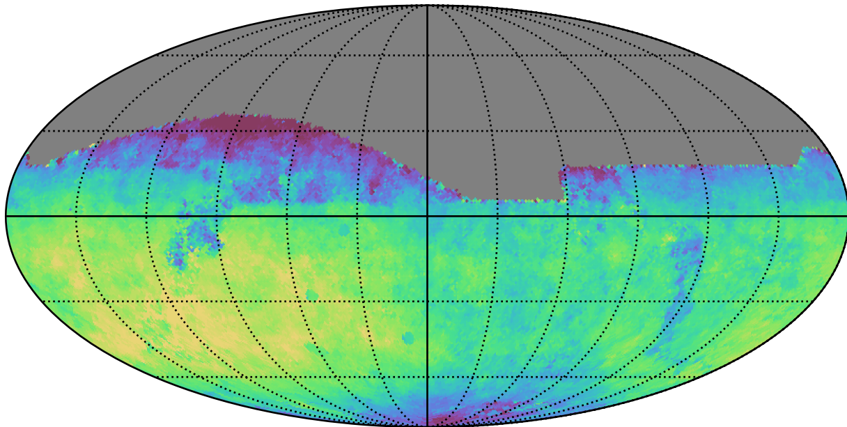
no_high_blob_v3.3_10yrs All sky z band: Median saturation_mag
