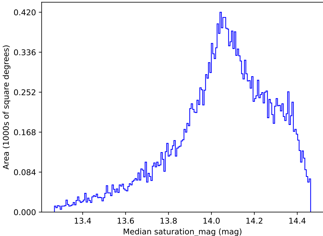
no_high_blob_v3.3_10yrs All sky z band: Median saturation_mag
