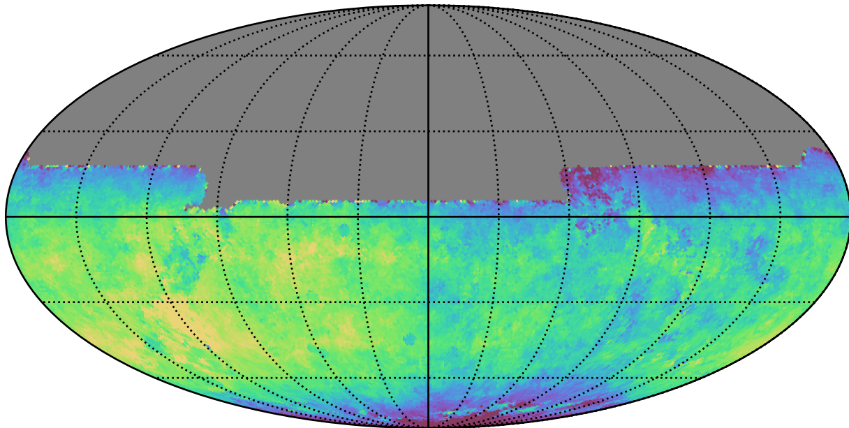
no_high_blob_v3.3_10yrs All sky y band: Median saturation_mag
