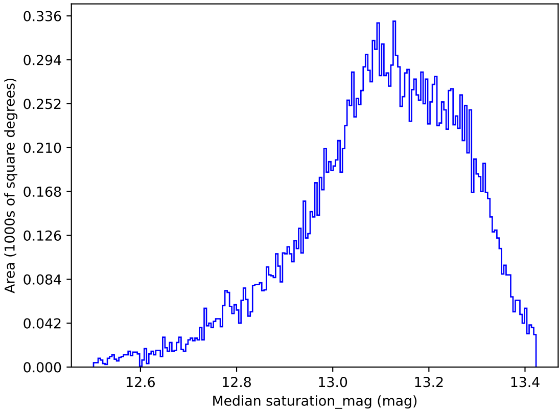
no_high_blob_v3.3_10yrs All sky y band: Median saturation_mag
