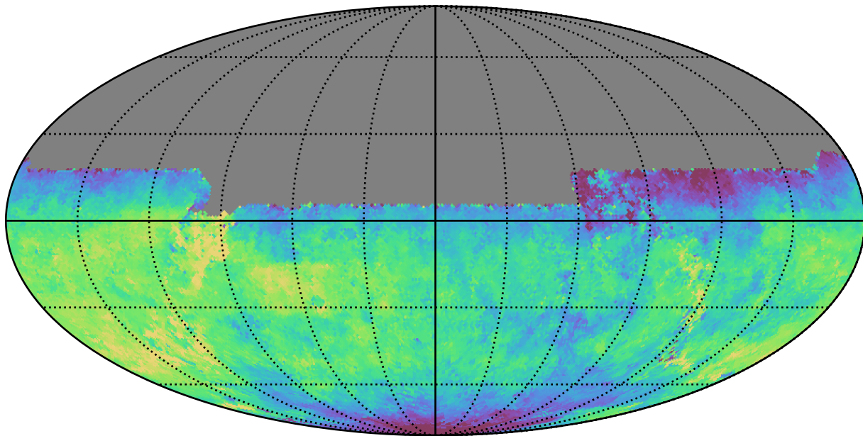
no_high_blob_v3.3_10yrs All sky u band: Median saturation_mag
