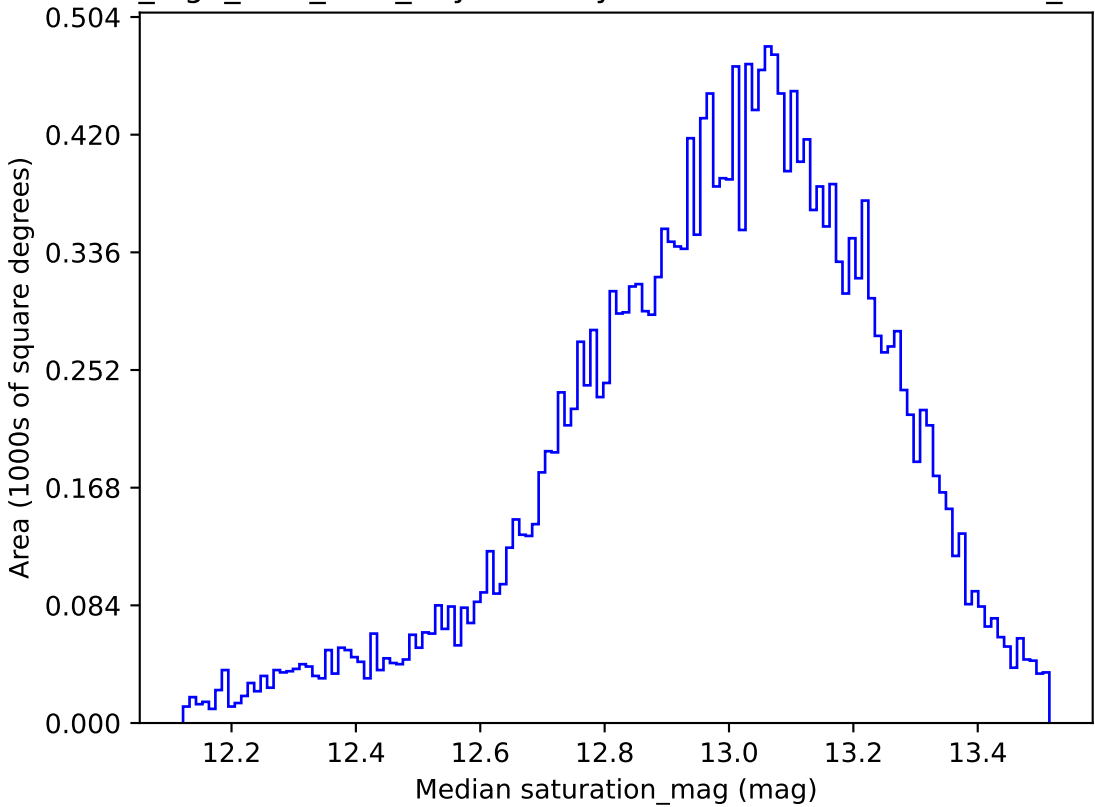
no_high_blob_v3.3_10yrs All sky u band: Median saturation_mag
