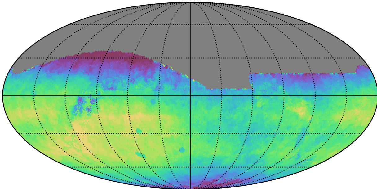
no_high_blob_v3.3_10yrs All sky r band: Median saturation_mag
