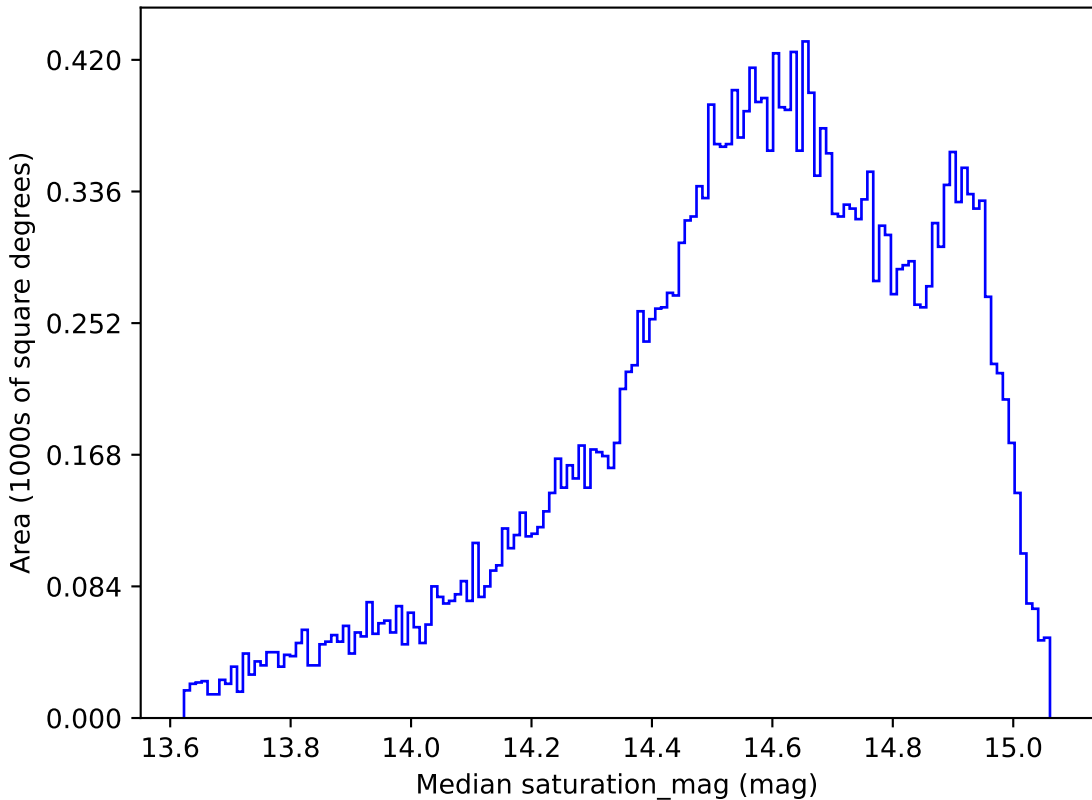
no_high_blob_v3.3_10yrs All sky r band: Median saturation_mag
