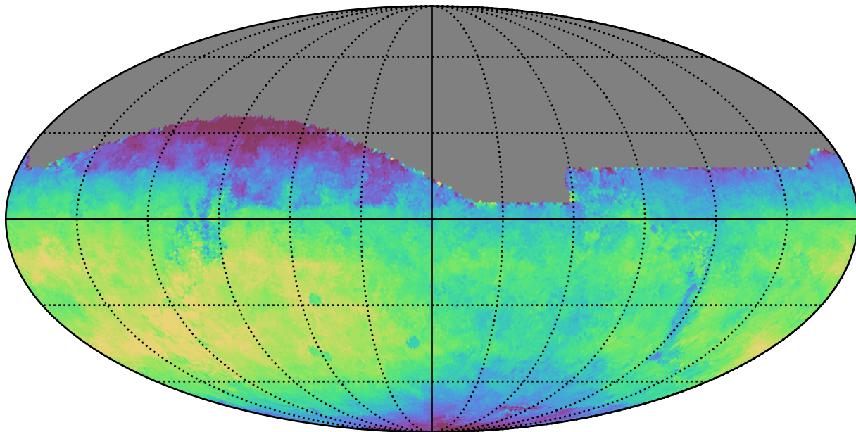
no_high_blob_v3.3_10yrs All sky i band: Median saturation_mag
