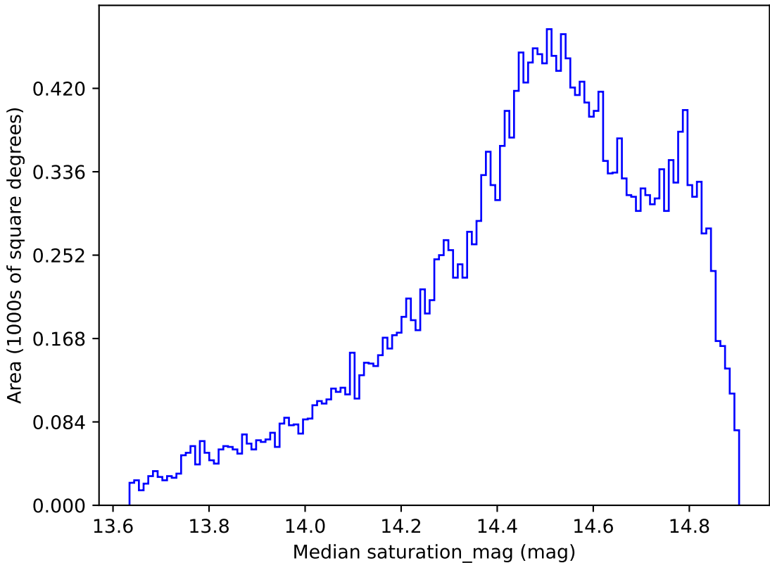
no_high_blob_v3.3_10yrs All sky i band: Median saturation_mag
