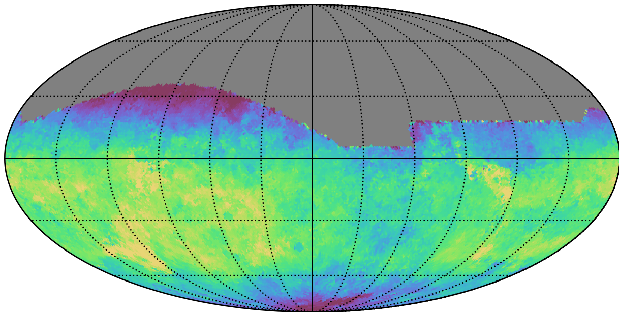
no_high_blob_v3.3_10yrs All sky g band: Median saturation_mag
