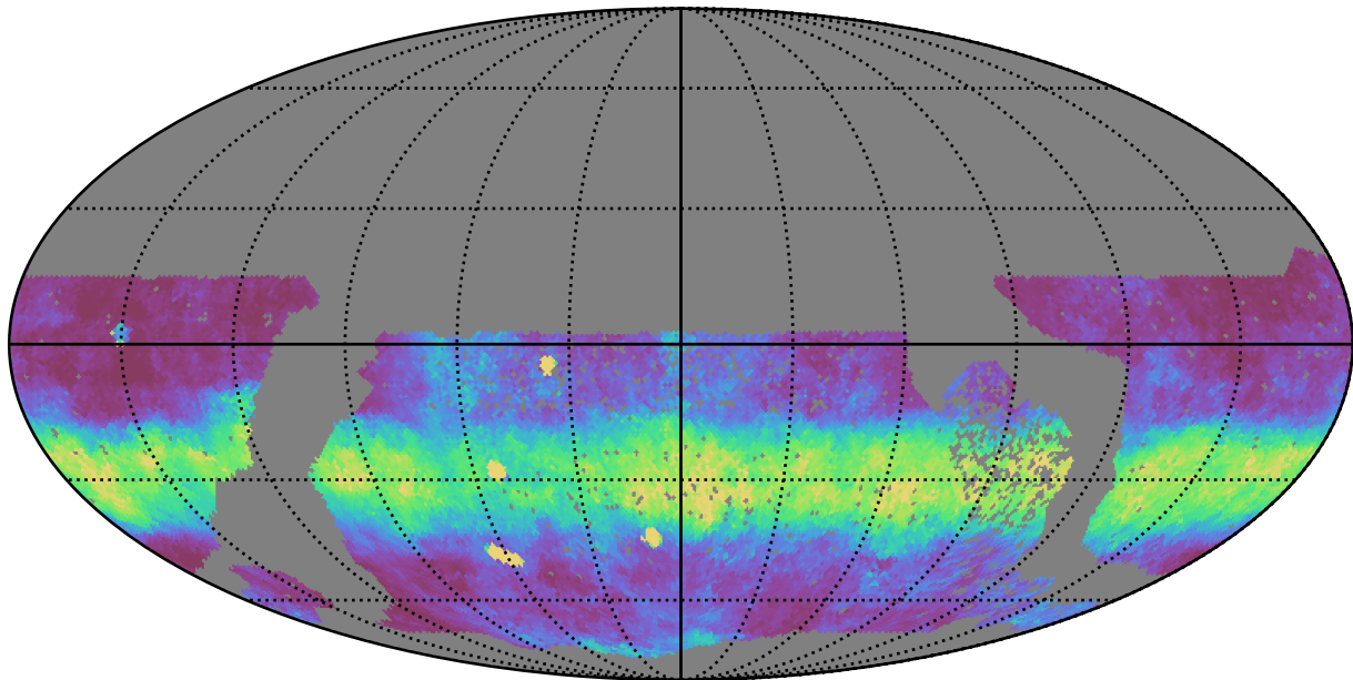
no_high_blob_v3.3_10yrs WFD z band: Median normairmass
