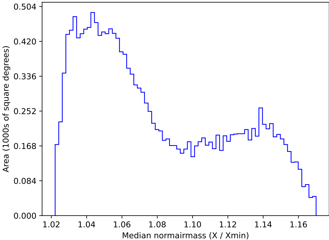
no_high_blob_v3.3_10yrs WFD z band: Median normairmass
