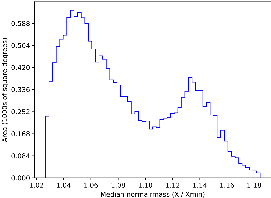
no_high_blob_v3.3_10yrs WFD y band: Median normairmass
