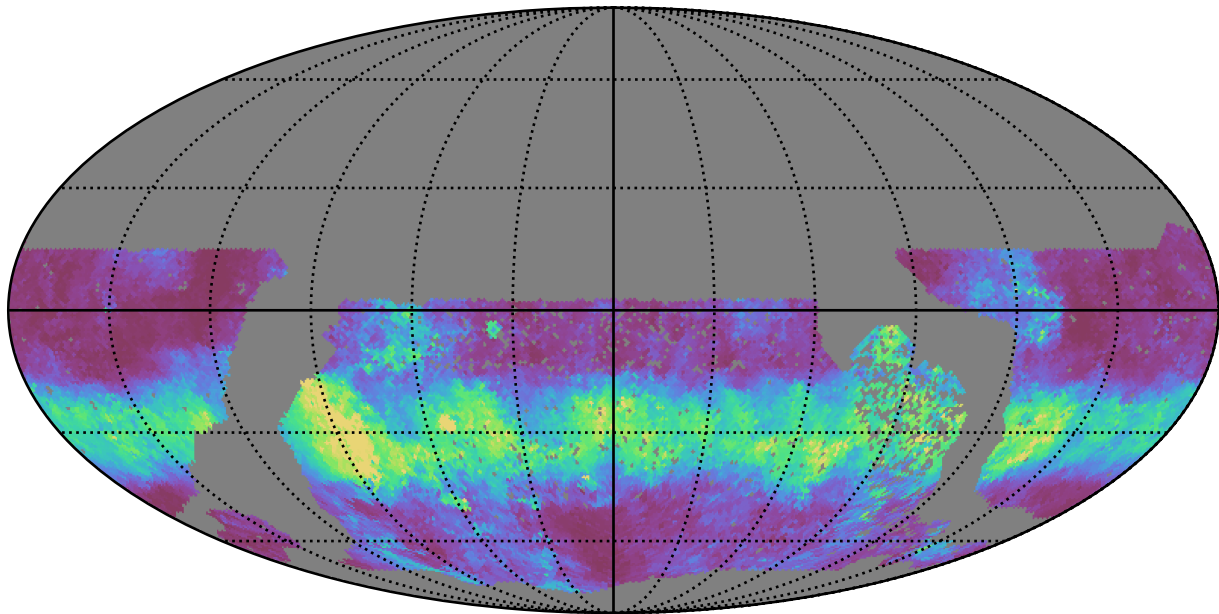
no_high_blob_v3.3_10yrs WFD u band: Median normairmass
