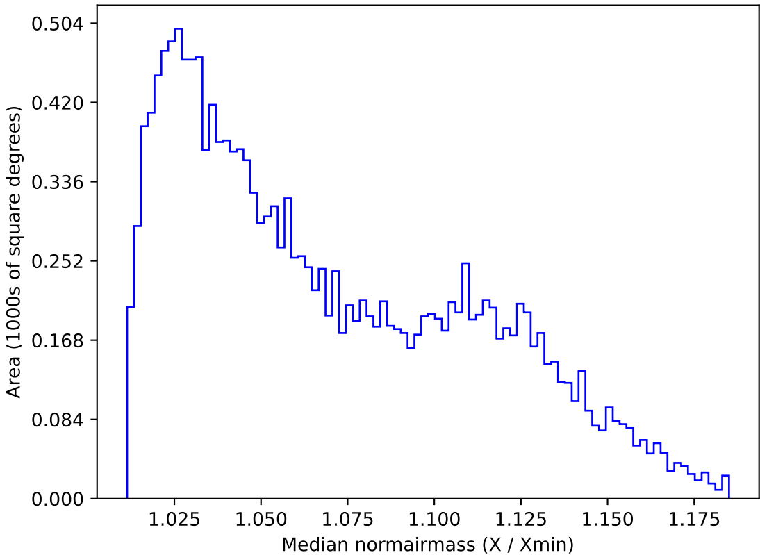
no_high_blob_v3.3_10yrs WFD u band: Median normairmass
