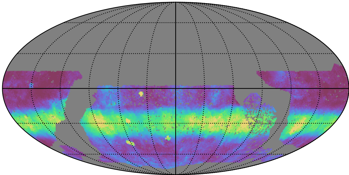
no_high_blob_v3.3_10yrs WFD r band: Median normairmass
