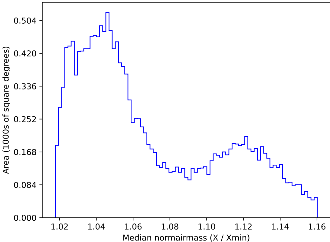
no_high_blob_v3.3_10yrs WFD r band: Median normairmass
