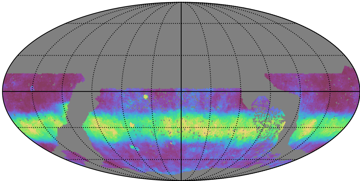
no_high_blob_v3.3_10yrs WFD i band: Median normairmass
