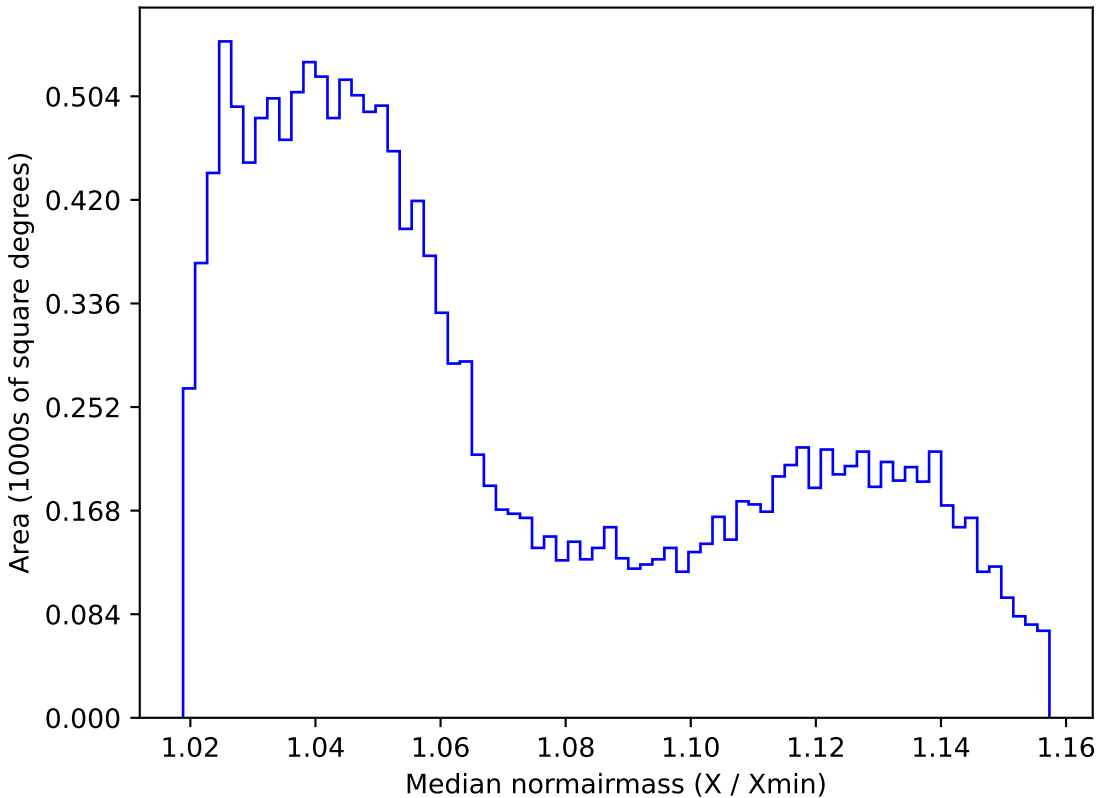
no_high_blob_v3.3_10yrs WFD i band: Median normairmass
