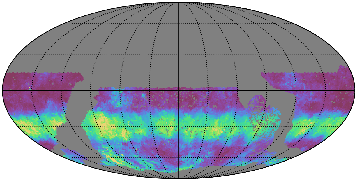
no_high_blob_v3.3_10yrs WFD g band: Median normairmass
