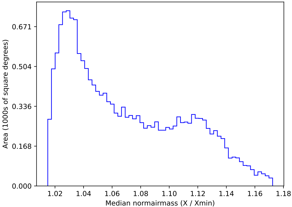
no_high_blob_v3.3_10yrs WFD g band: Median normairmass
