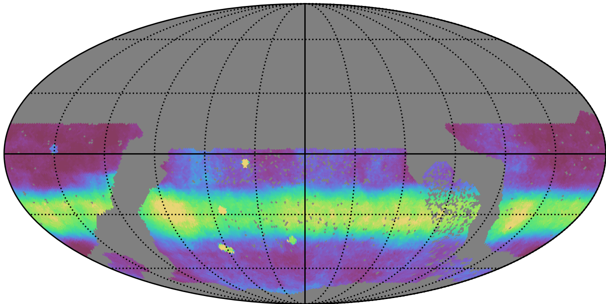
no_high_blob_v3.3_10yrs WFD all bands: Median normairmass
