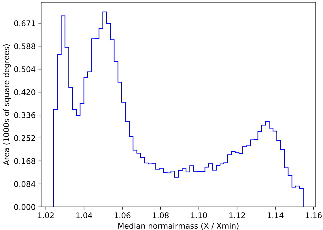
no_high_blob_v3.3_10yrs WFD all bands: Median normairmass
