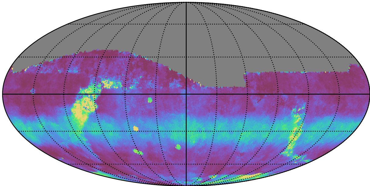
no_high_blob_v3.3_10yrs All sky z band: Median normairmass
