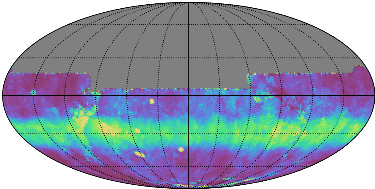
no_high_blob_v3.3_10yrs All sky y band: Median normairmass
