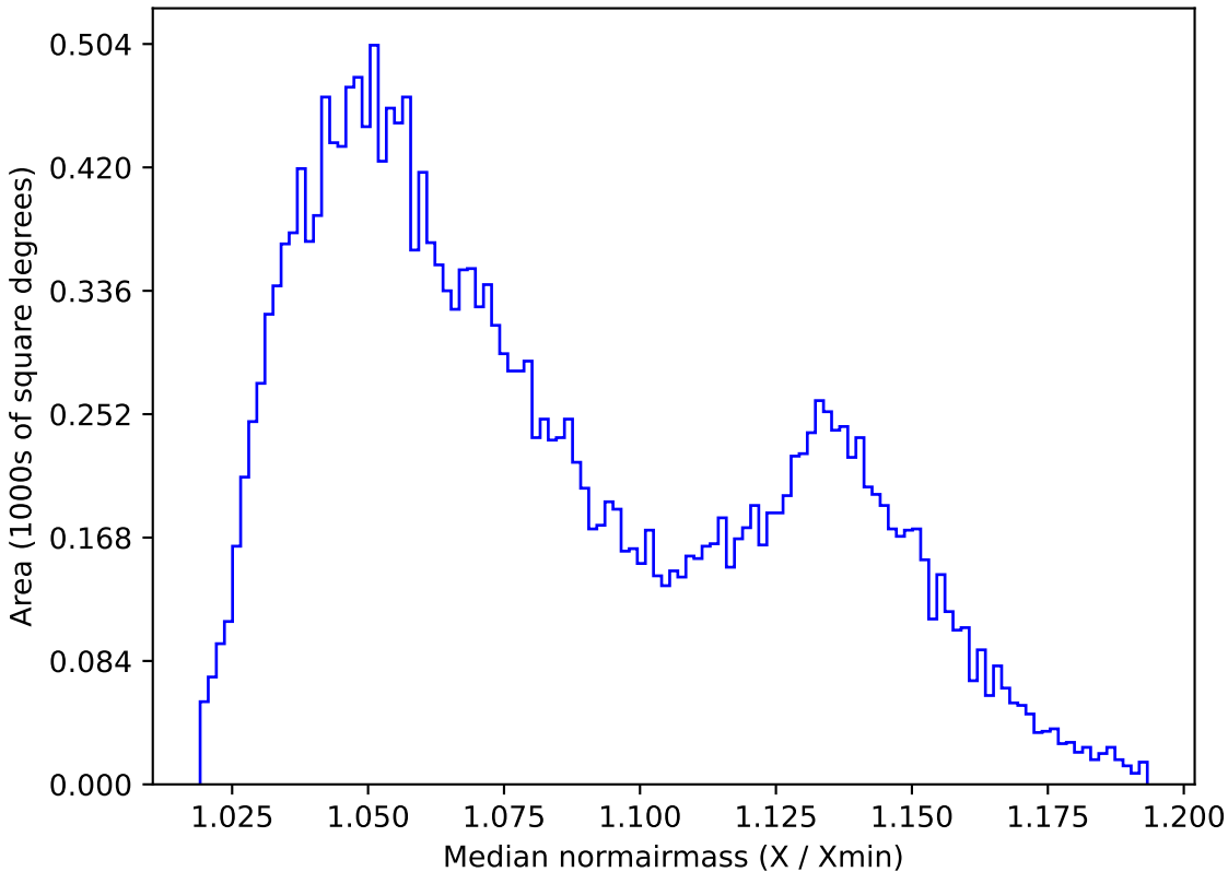
no_high_blob_v3.3_10yrs All sky y band: Median normairmass
