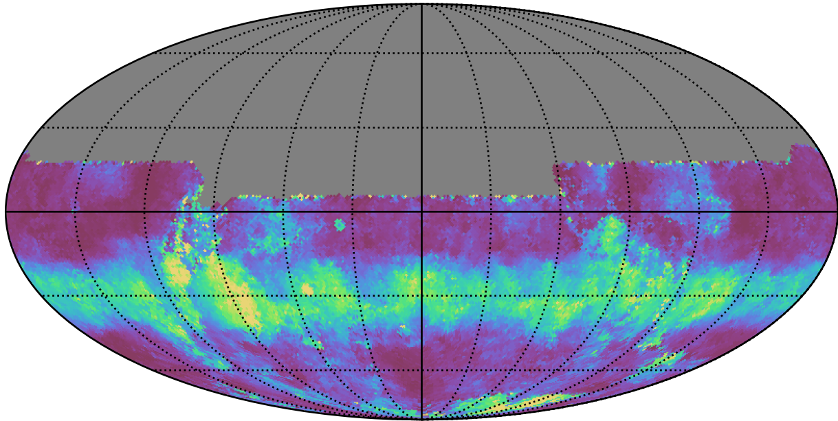
no_high_blob_v3.3_10yrs All sky u band: Median normairmass
