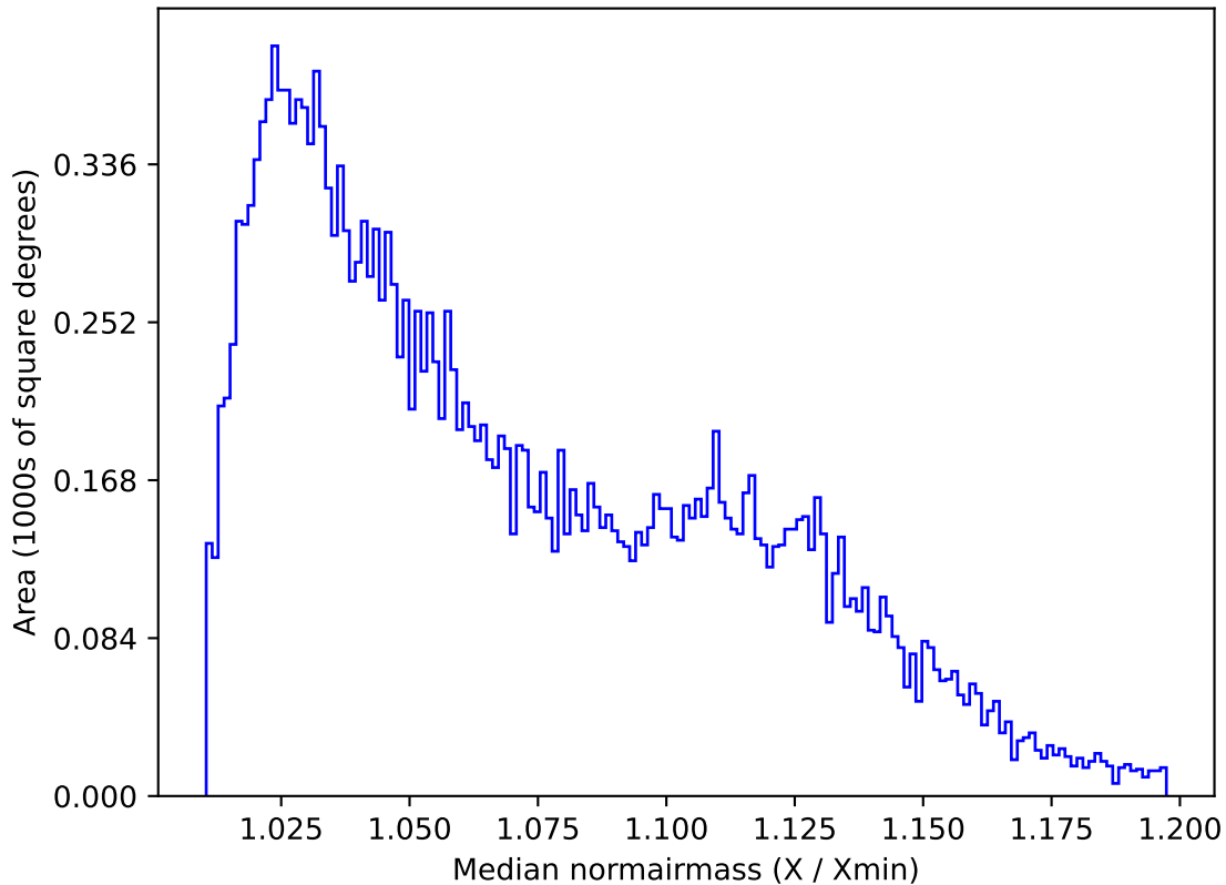
no_high_blob_v3.3_10yrs All sky u band: Median normairmass
