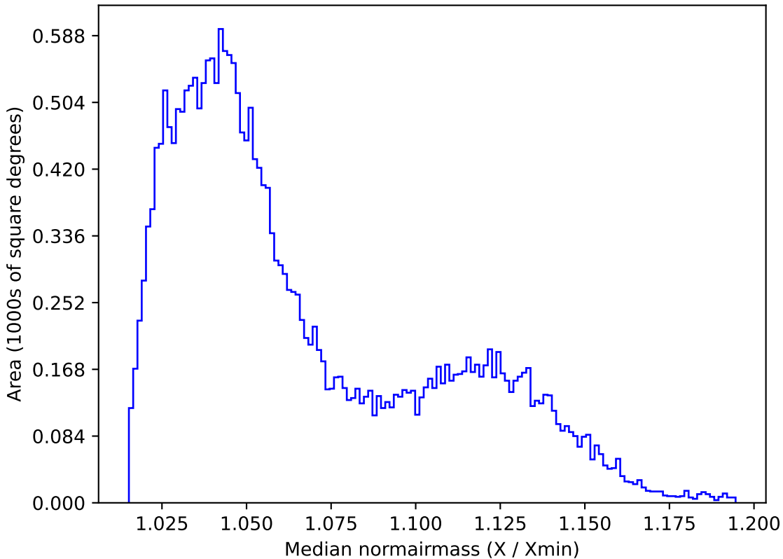
no_high_blob_v3.3_10yrs All sky r band: Median normairmass
