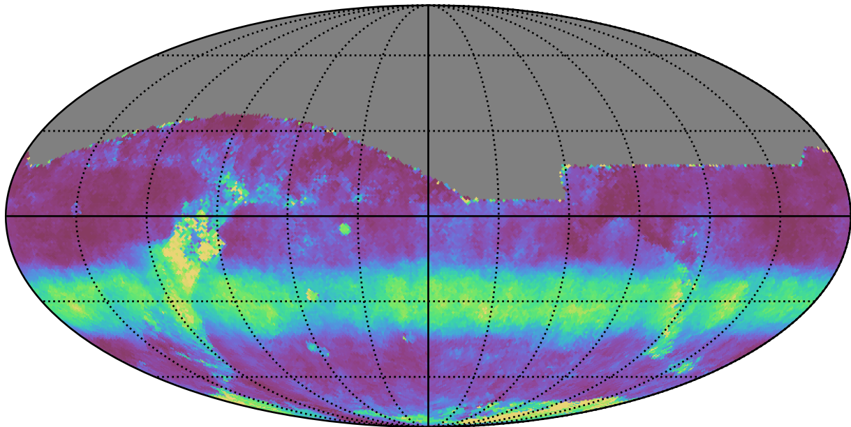
no_high_blob_v3.3_10yrs All sky i band: Median normairmass
