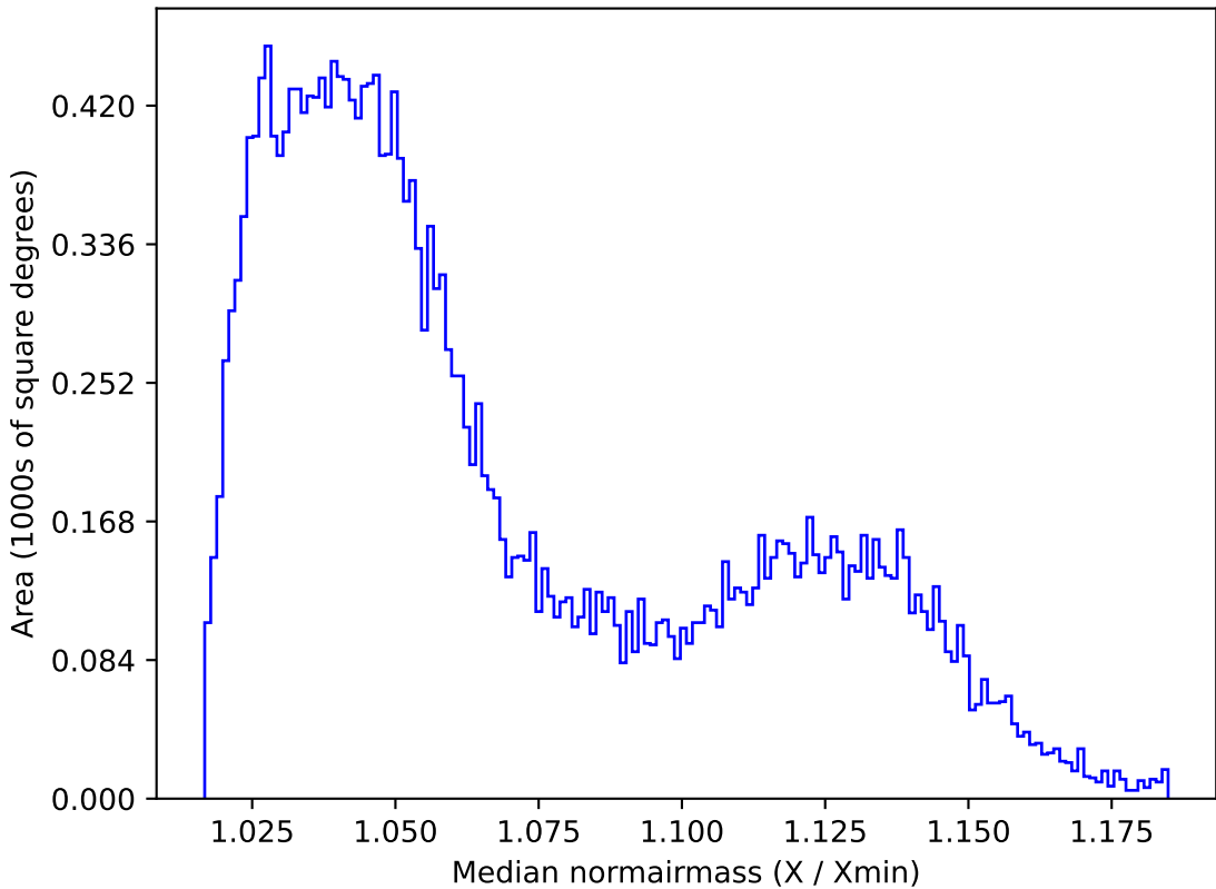
no_high_blob_v3.3_10yrs All sky i band: Median normairmass
