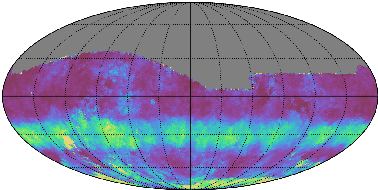
no_high_blob_v3.3_10yrs All sky g band: Median normairmass
