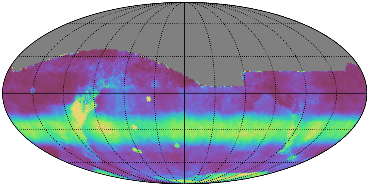
no_high_blob_v3.3_10yrs All sky all bands: Median normairmass
