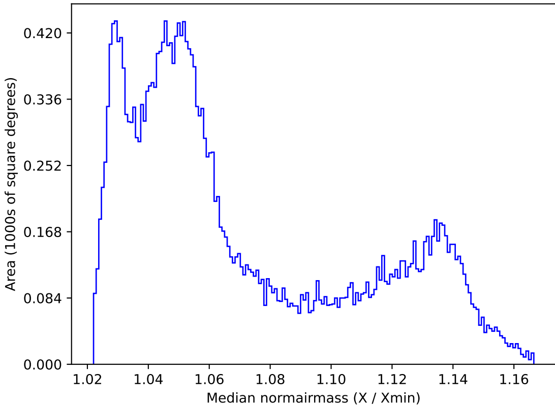
no_high_blob_v3.3_10yrs All sky all bands: Median normairmass
