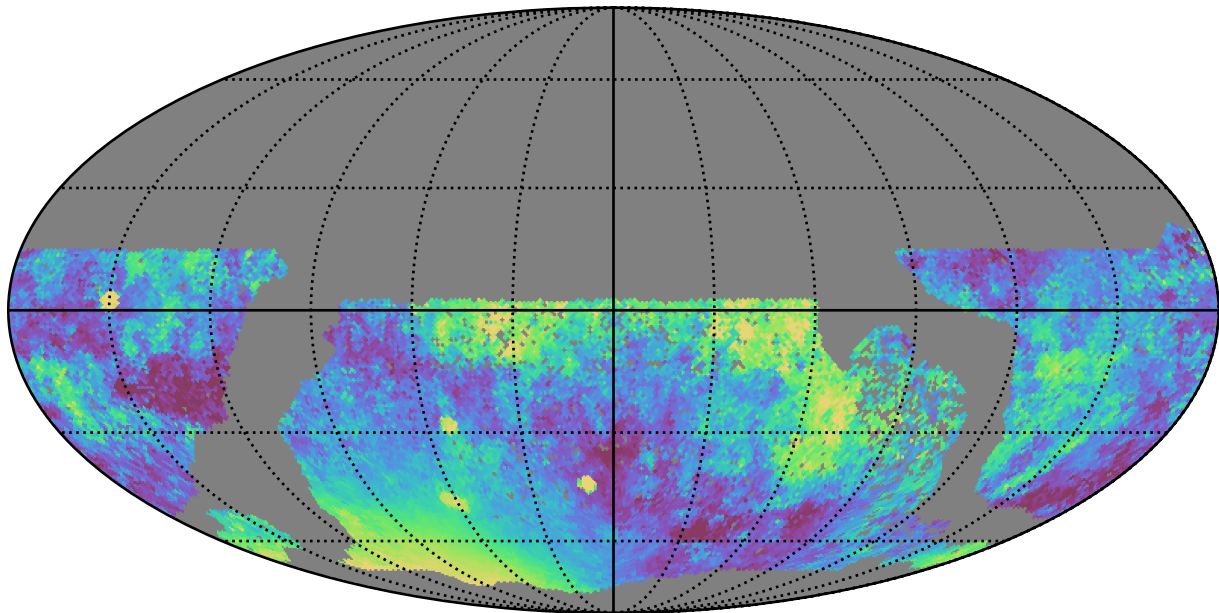
no_high_blob_v3.3_10yrs WFD z band: Median moonDistance
