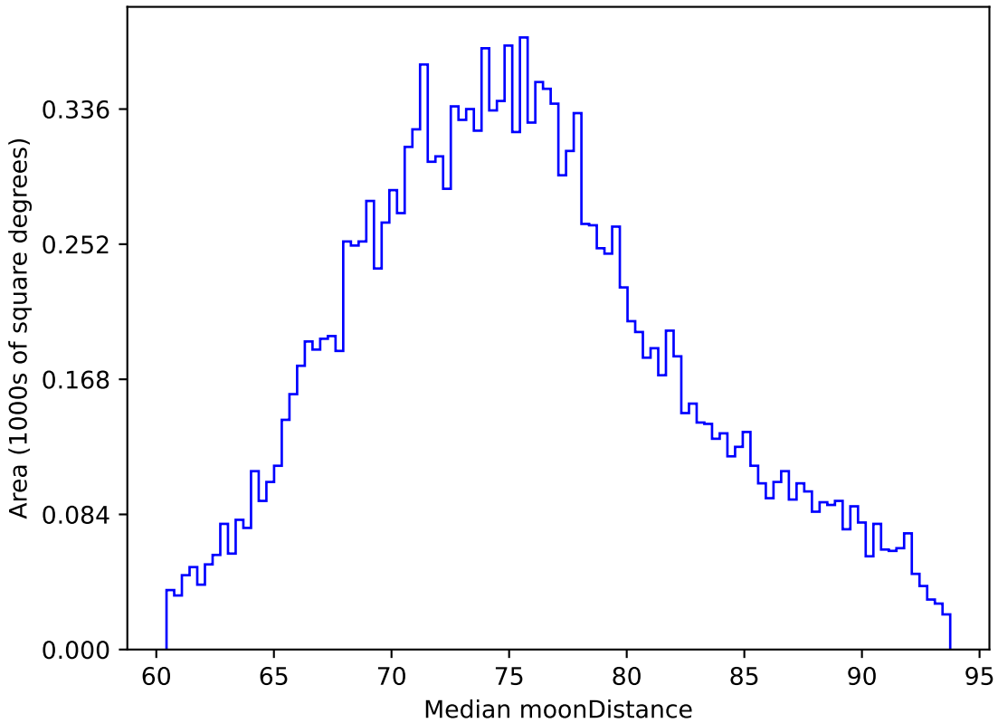
no_high_blob_v3.3_10yrs WFD z band: Median moonDistance
