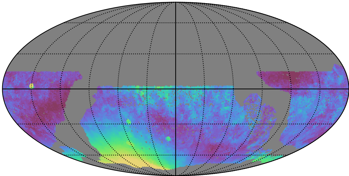
no_high_blob_v3.3_10yrs WFD y band: Median moonDistance
