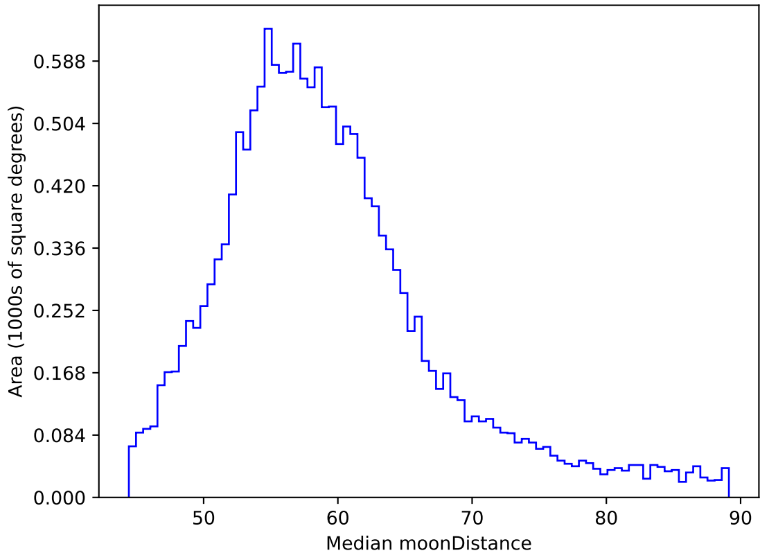
no_high_blob_v3.3_10yrs WFD y band: Median moonDistance
