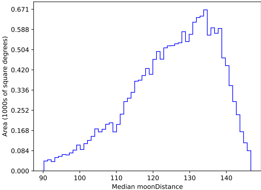
no_high_blob_v3.3_10yrs WFD u band: Median moonDistance
