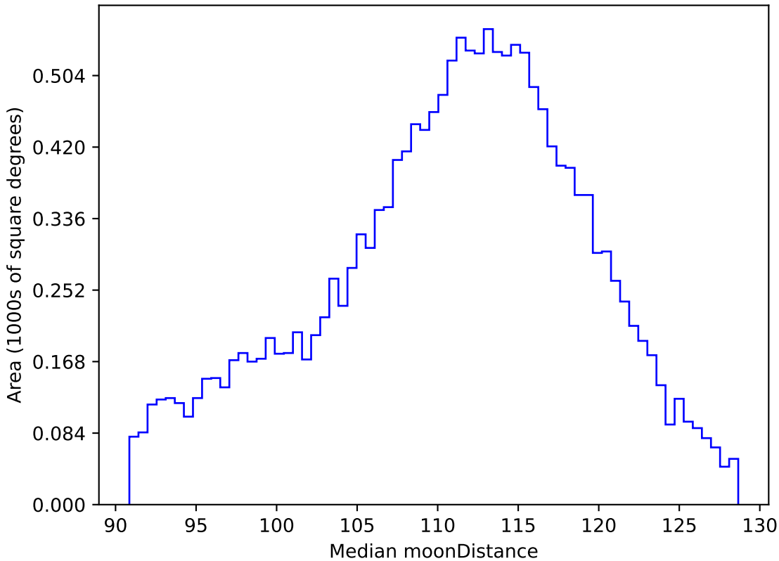
no_high_blob_v3.3_10yrs WFD r band: Median moonDistance
